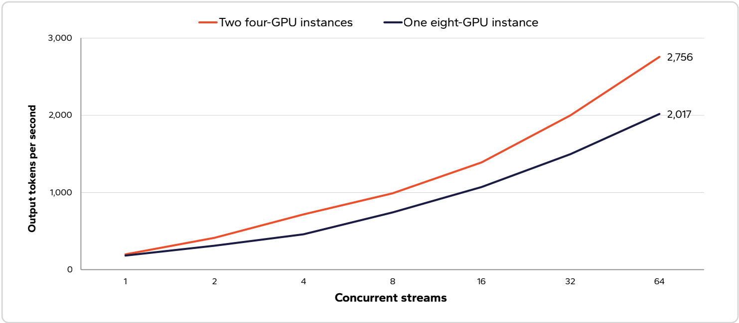
Figure 2: Aggregate output throughput as simultaneous streams increase
