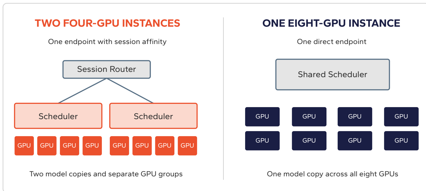
Figure 1: Two deployment layouts on the same eight-GPU server
