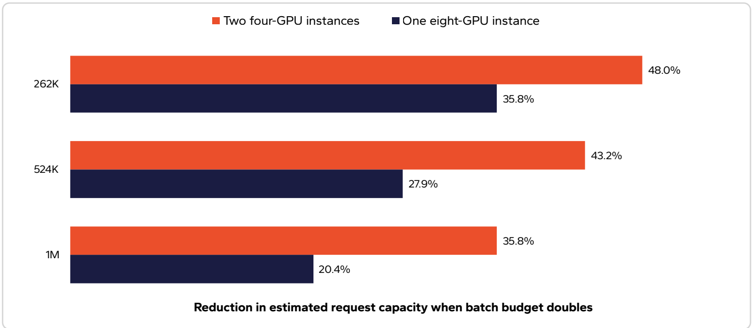
Figure 5: Reduction in estimated request capacity when the batch budget doubled
