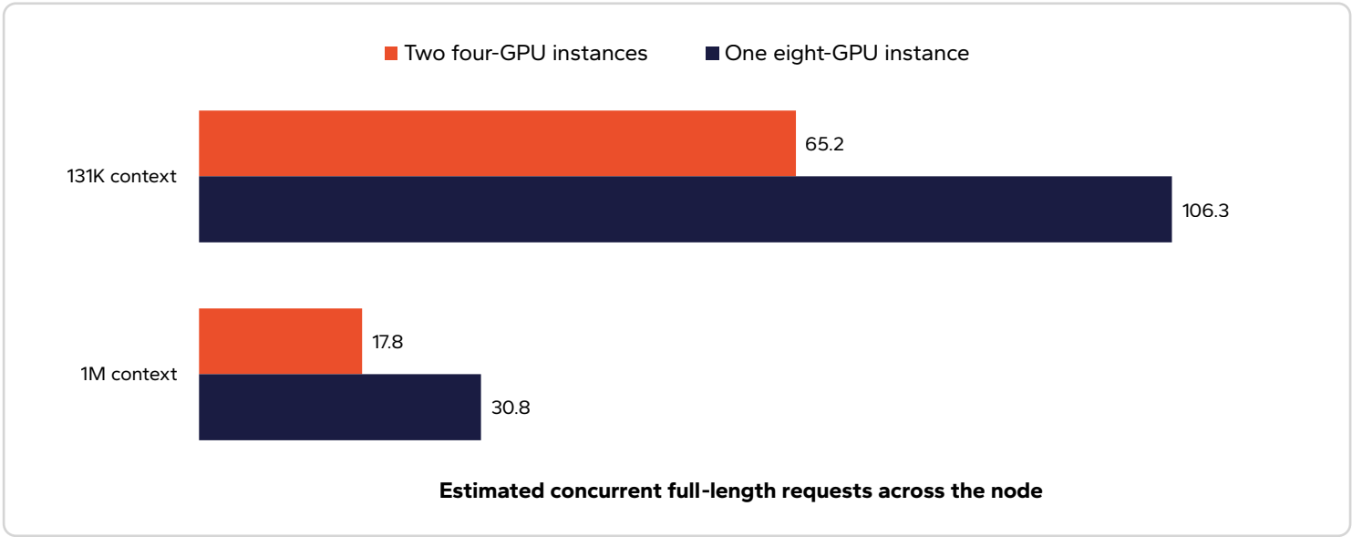
Figure 4: Estimated capacity for full-length requests at matched context ceilings
