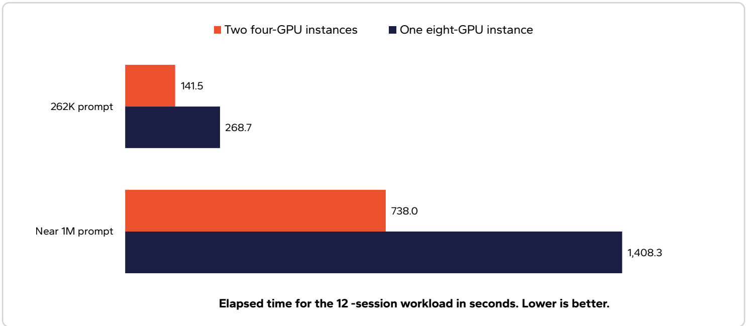
Figure 3: Elapsed time for 12 concurrent long-context sessions
