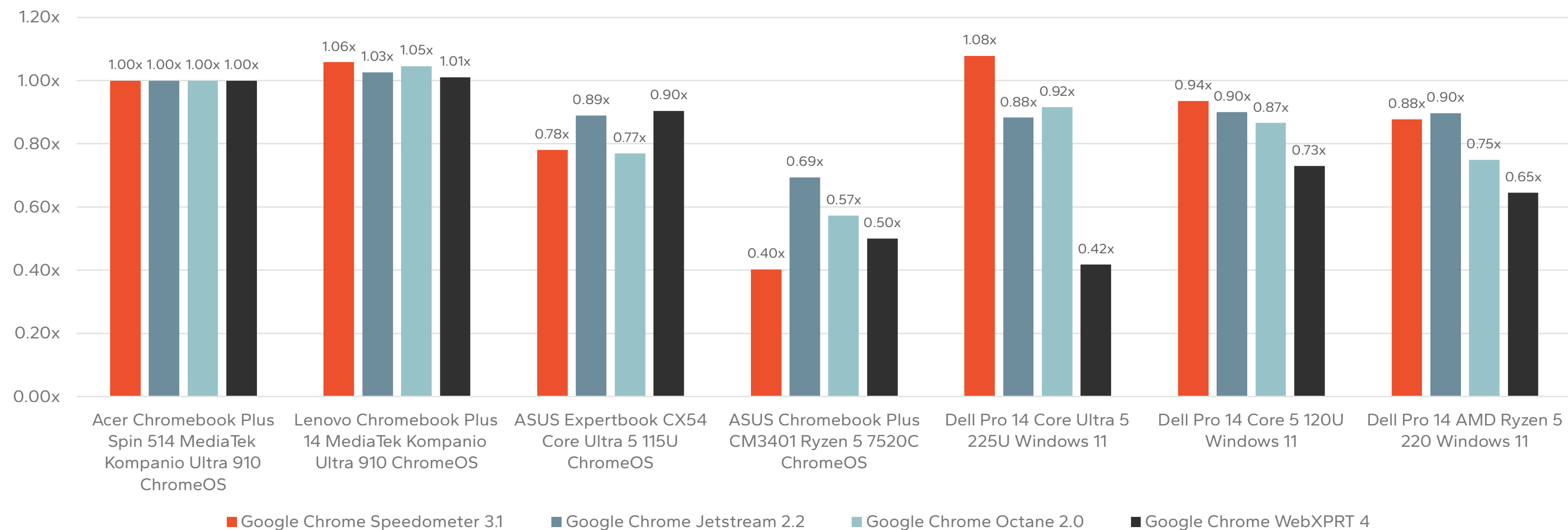
DC Performance - Google Chrome Browser Tests
